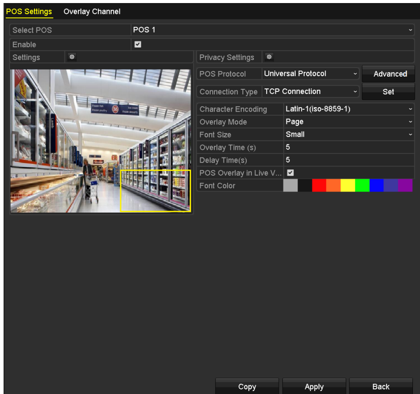
Figure 9-1 POS Settings
