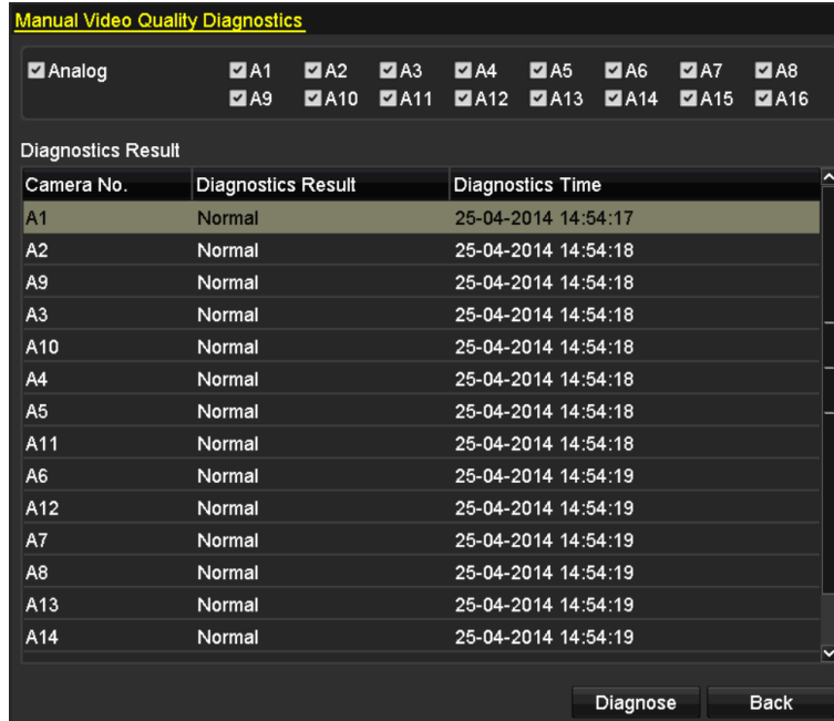
Figure 3-14 Diagnostics Result
