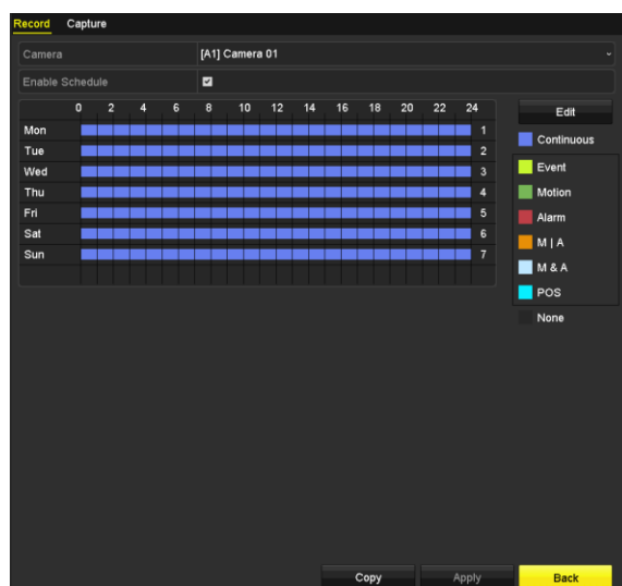
Figure 5-8 Record Schedule
